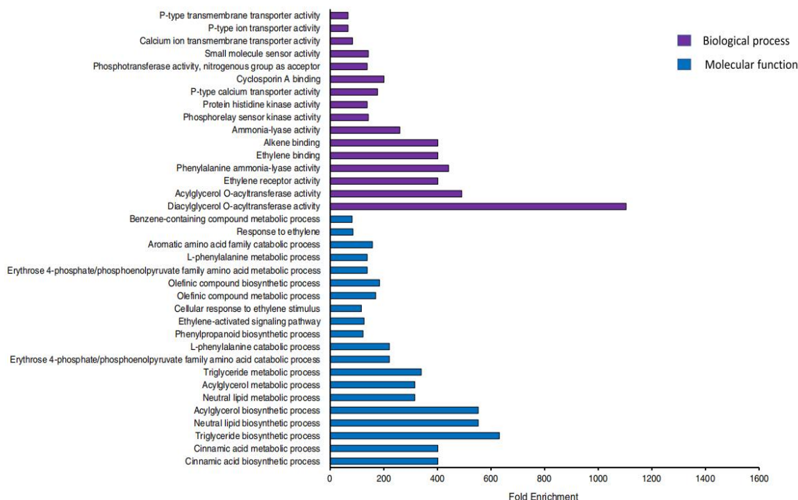
Figure 2 Gene ontology (GO) enriched terms associated with differentially expressed genes (DEGs) in starch content (Ruanjaichon et al., 2021)
